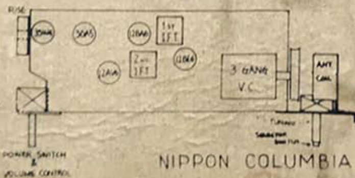
PART LOCATION
