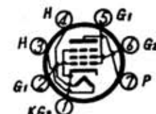
50C5
