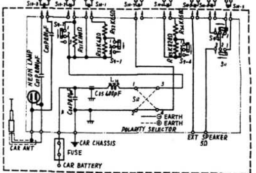
RD-884CA CAR BRACKET SECTION
