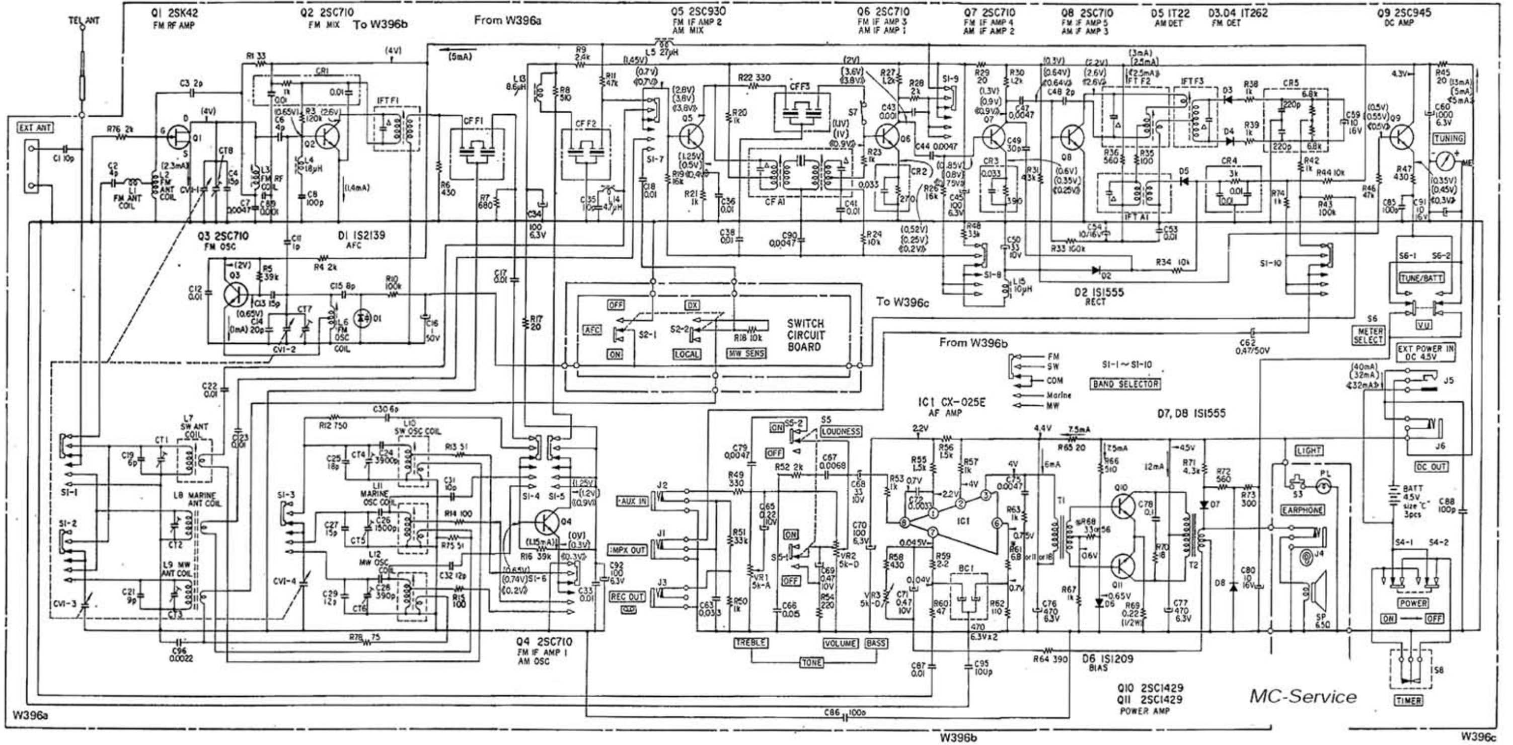
CIRCUIT DIAGRAM—MODEL ICF-5500M
