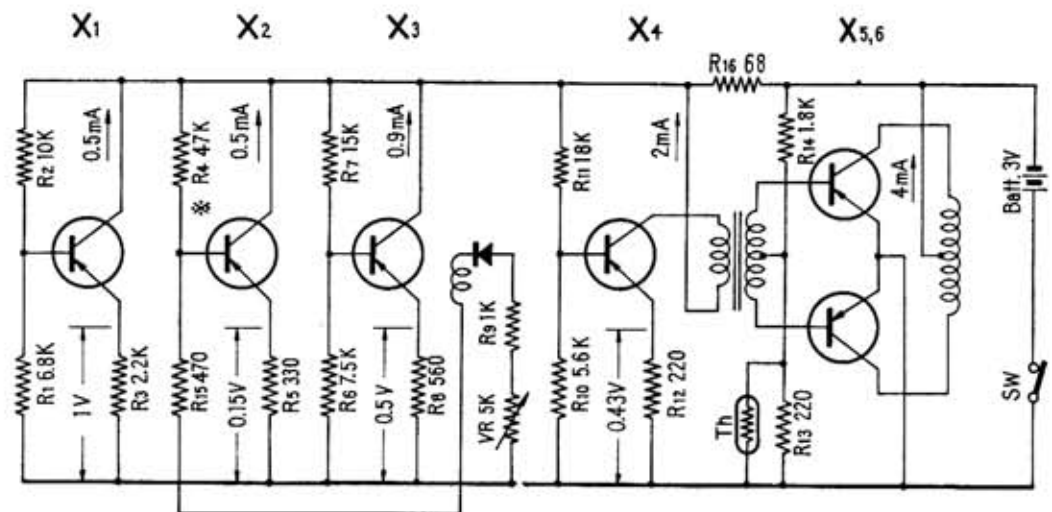
Voltage and Current Distribution Chart at Zero Signal
