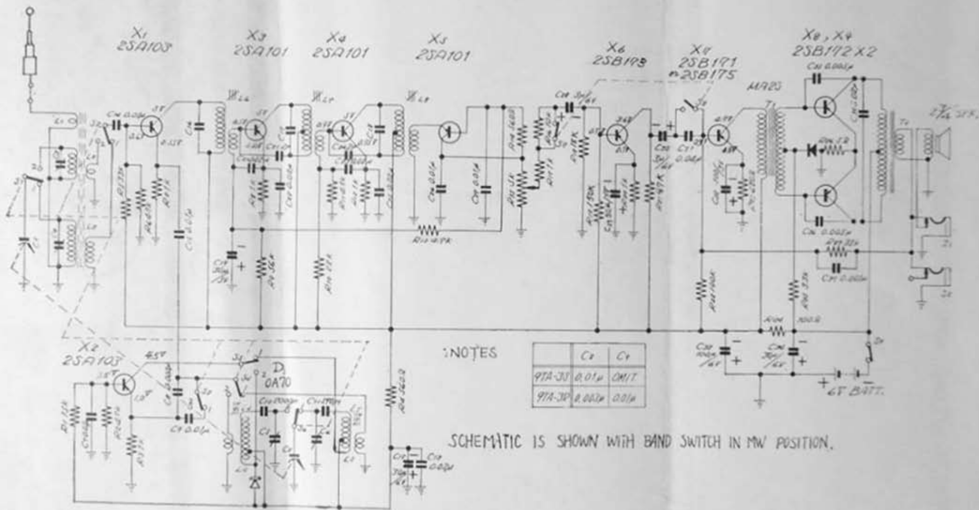
SCHEMATIC DIAGRAM MODEL 9TA-3S 9TA-3R
